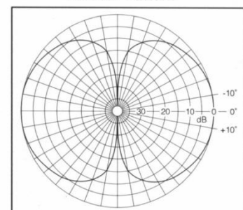
Vertical Pattern
